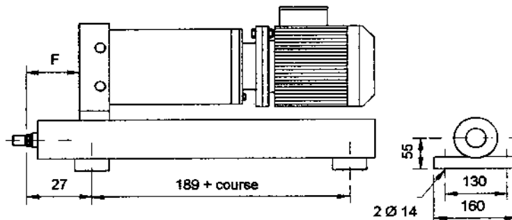
Support tourillon TB-25
